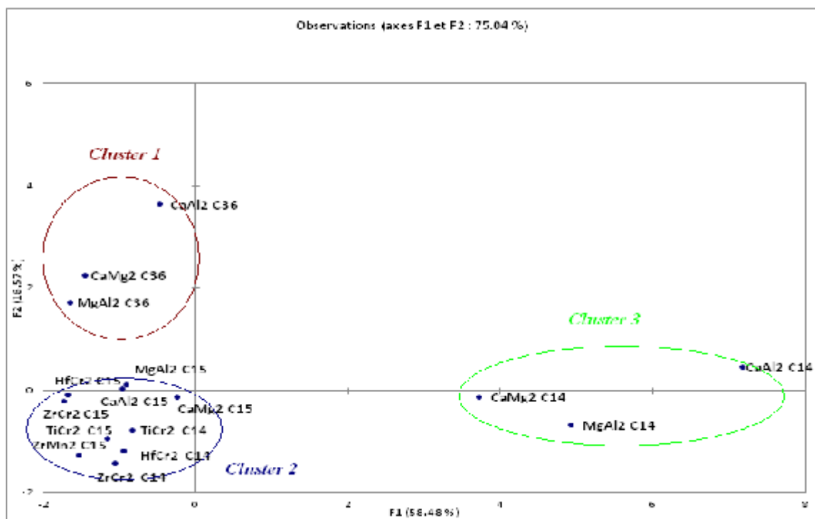
Figure (III-2) : graphe des observations (scores plot).
